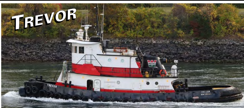
1,700 HP Model Bow Tug • 1978 • Length: 69' Beam: 26' • Depth: 9.6' • Main Engines: (2) Cat C32 - Tier 2 Sale Price: $1,300,000.00 • Location: U.S. East Coast
