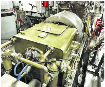
(2) FALK 12 MB GEARS 2.028:1 RATIO
